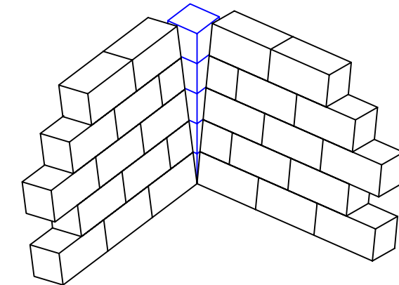
90° CORNER -WITH BATTER (MSE WALL)
