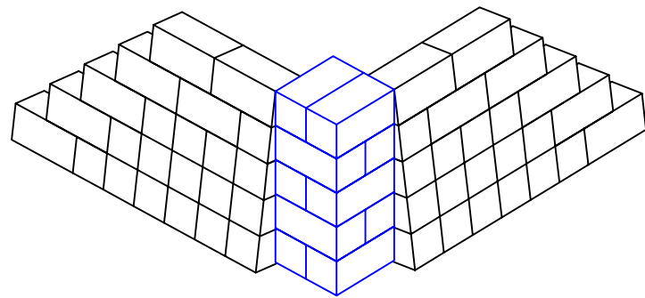
OUTSIDE 90 (GRAVITY WALL)
