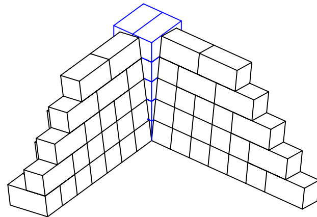
INSIDE ANGLE (GRAVITY WALL)
