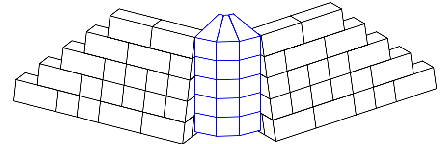
OUTSIDE ANGLE (GRAVITY WALL)
