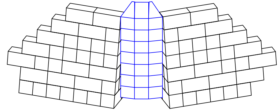
OUTSIDE ANGLE (GRAVITY WALL)
