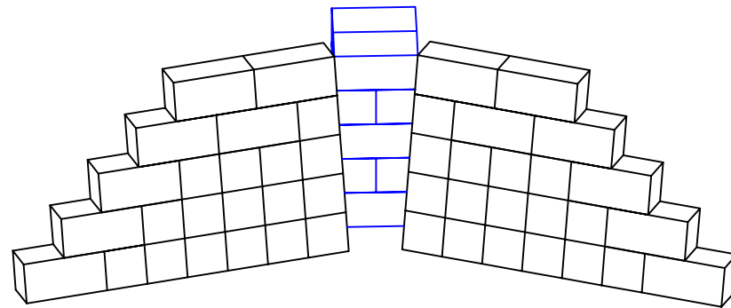
INSIDE ANGLE (GRAVITY WALL)
