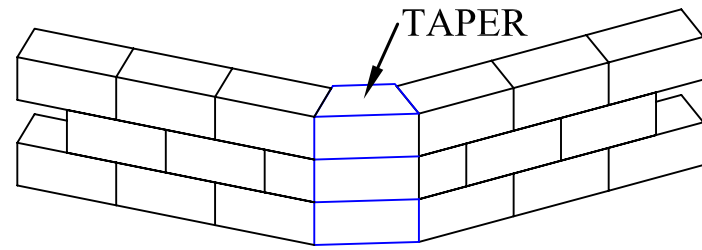
OUTSIDE ANGLE -NO BATTER (MSE WALL)
